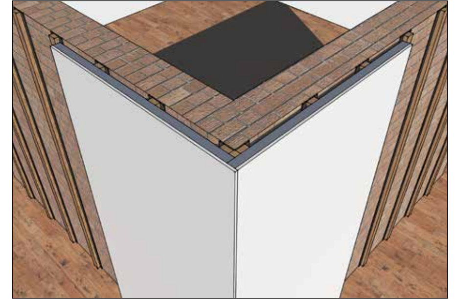
Fig. 5 External Angle Joint in Spacetherm Wallboard
