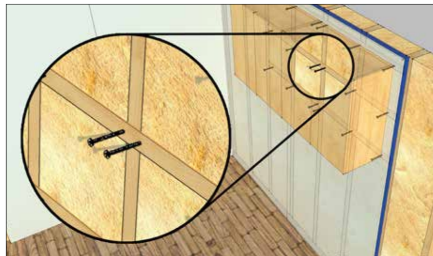
Fig. 9 Fixing kitchen units through Spacetherm Multi / A2 Multi
