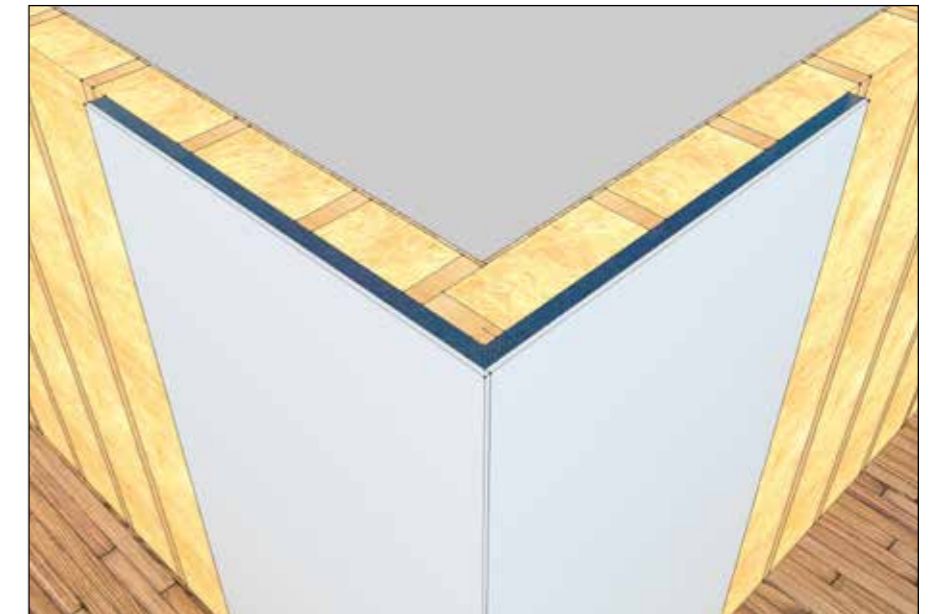
Fig. 5 External Angle Joint in Spacetherm Multi / A2 Multi
