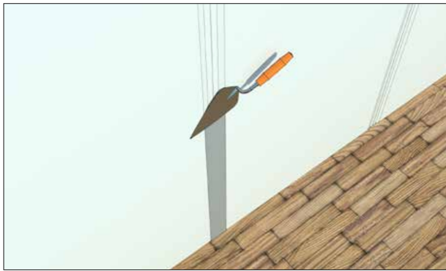
Fig. 8 Taping and Filling Joints in Spacetherm Multi / A2 Multi
