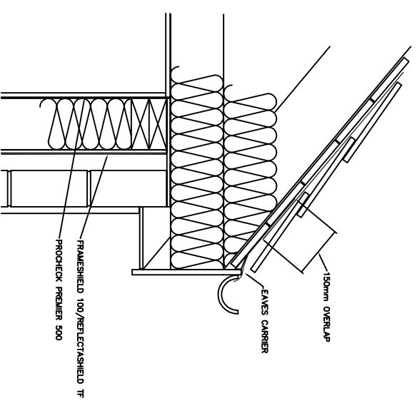
SCOTTISH COLD ROOF SW SARKING
